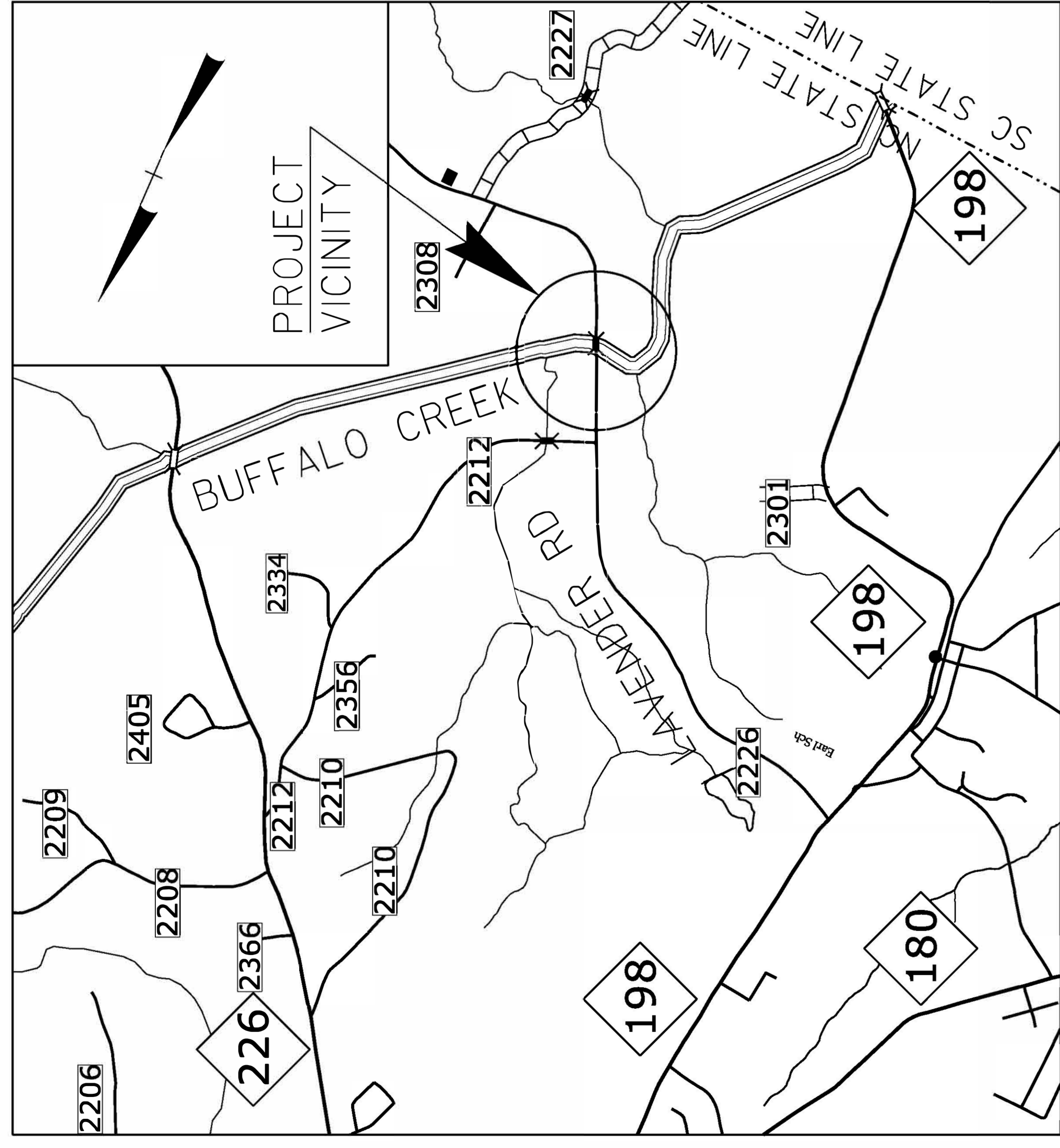
VICINITY MAP
